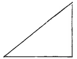
rectangulum
