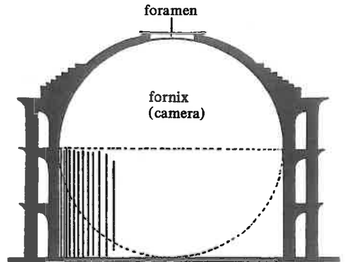
orthographia Pantheonis
